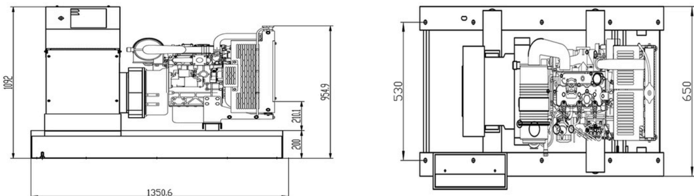
Open Type (without Soundproof Canopy)
