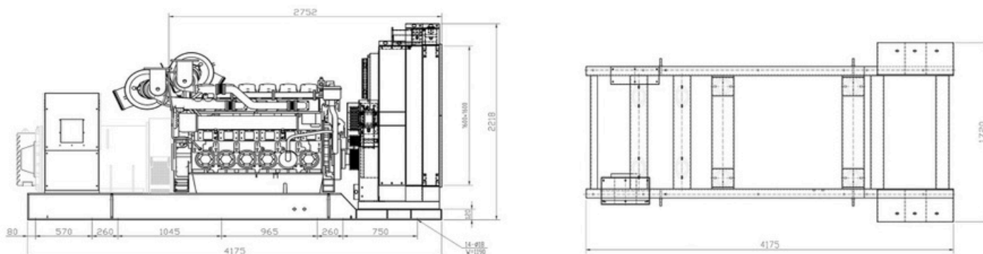
Open Type (without Soundproof Canopy)
